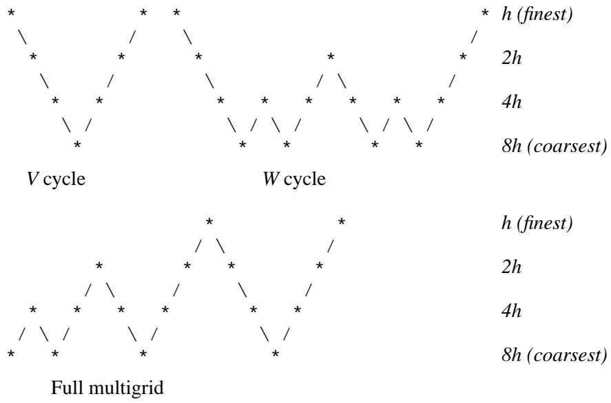
Figure 11.8 Patterns for multigrid methods.
