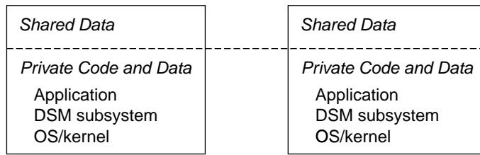
Figure 10.15 Structure of a distributed shared memory system.
