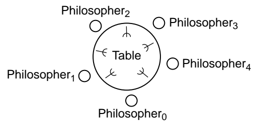
Figure 4.6 The dining philosophers.
