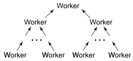
Figure 3.13 Tree-structured barrier.
