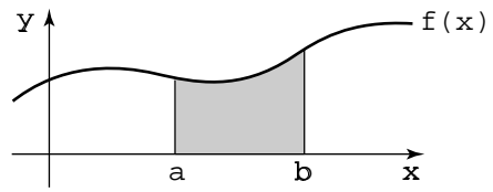
Figure 1.4 The quadrature problem.
