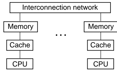
Figure 1.3 Structure of distributed-memory machines.
