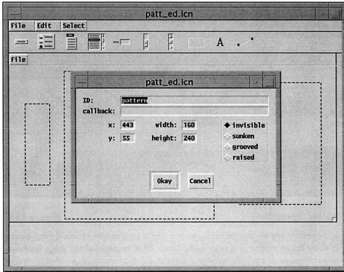
The Interface as Seen in VIB
