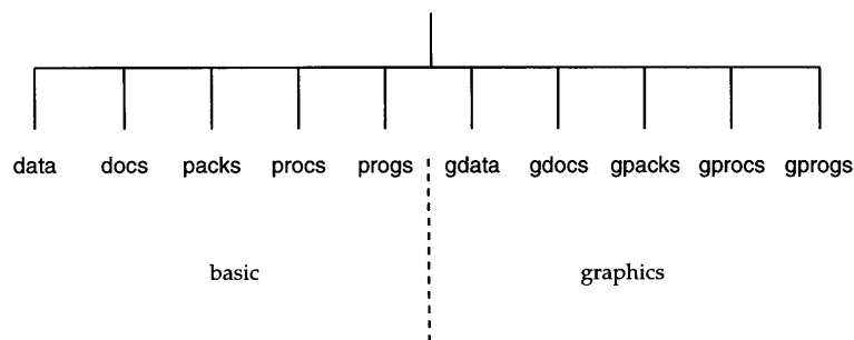
Icon Program Library Hierarchy
