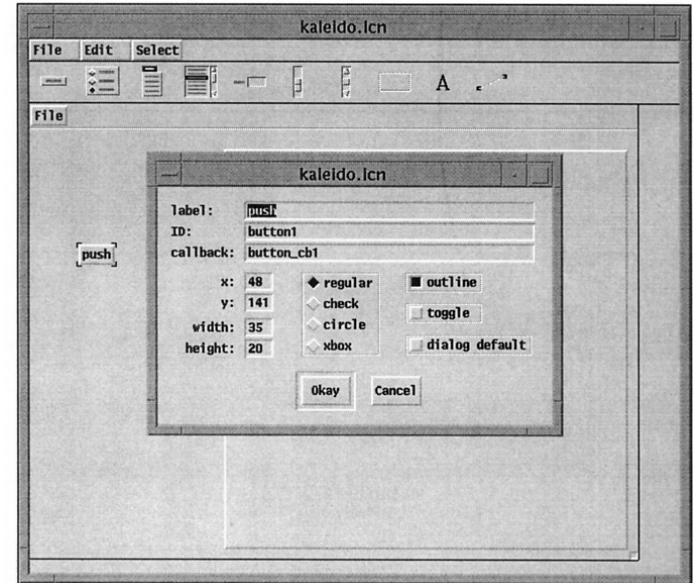
A Button Dialog
