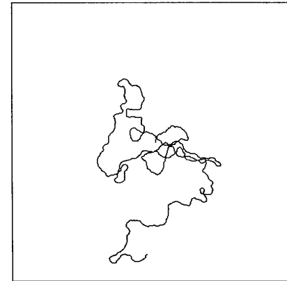
A Random Walk
