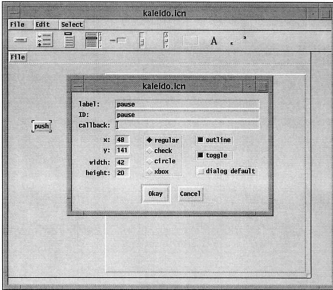
The Edited Button Dialog
