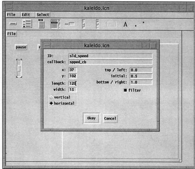
The Edited Slider Dialog
