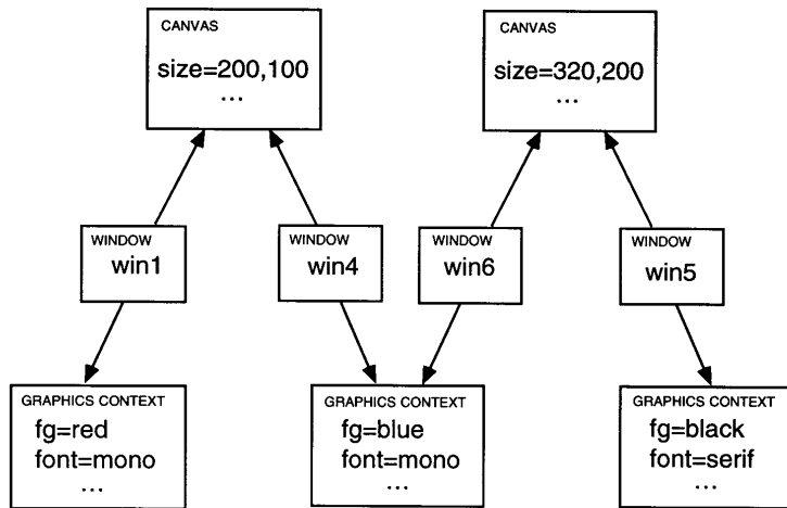
Shared Graphics Contexts
