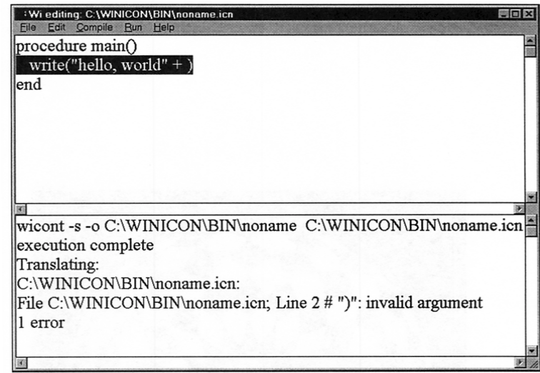
A Syntactic Error
