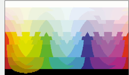
The c6 Surface
